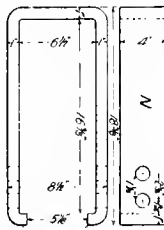
Figs. 5528-5529. YOKE OR STRAP-POCKET. RECOMMENDED PRACTICE IN ATTACHMENT OF COUPLERS.
